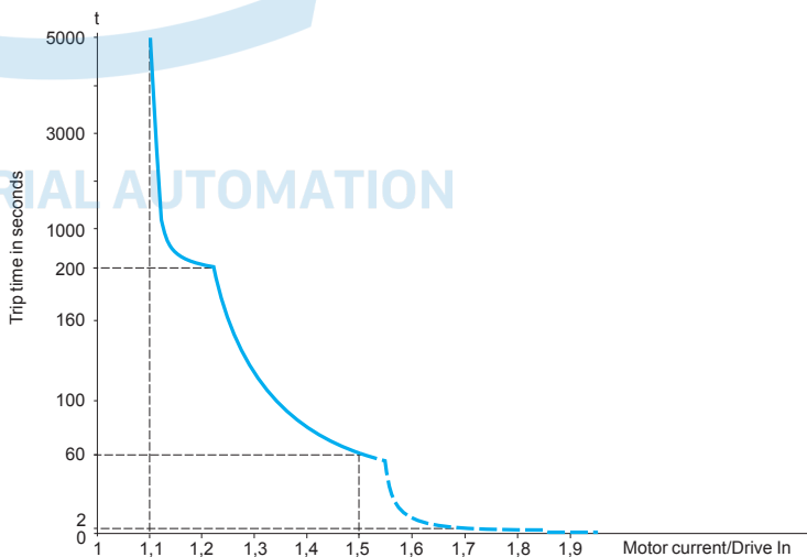
Drive thermal protection curves
