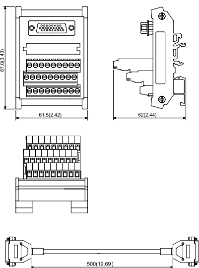
ACS3-MDTD2600 (for B3-M, F, and E)
