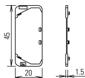
HW-VG1 Dual Pushbutton Barrier
