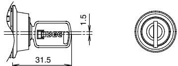
Key No.: 3H to 6H (non-reversible key)
