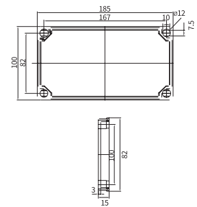
COVER
