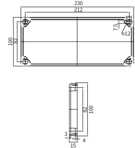
COVER
