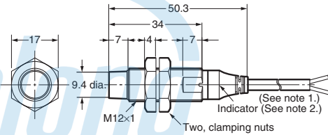
E2A-M12KN08-WP-□□
