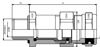
Metric Thread
