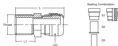
Metric Thread
