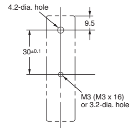
Mounting Hole Dimensions
