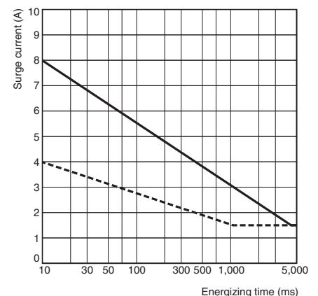
G3R-OD201SN (-UTU) (40 to 200 VDC)
