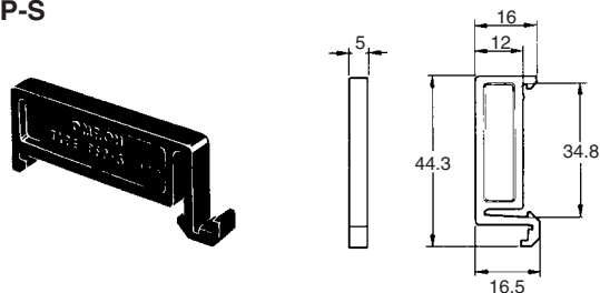
Spacer PFP-S
