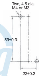
Mounting Holes
