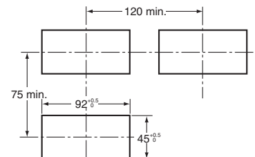
Panel cut-out
