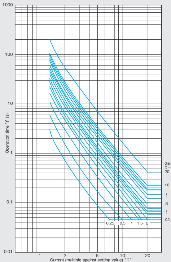
EI : Extremely inverse time-delayed characteristic
