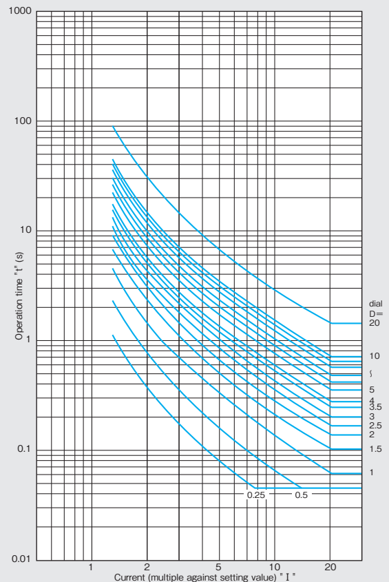
VI : Very inverse time-delayed characteristic
