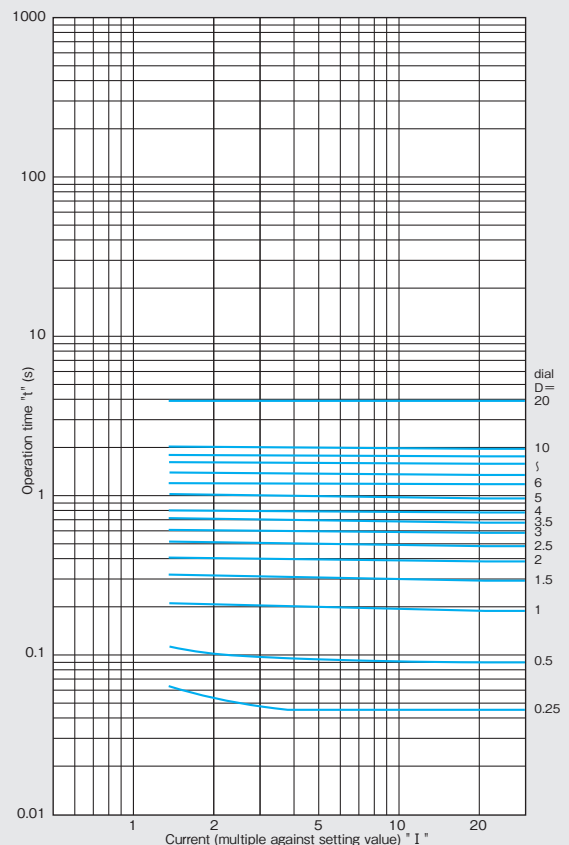
DT : Definite time-delayed characteristic
