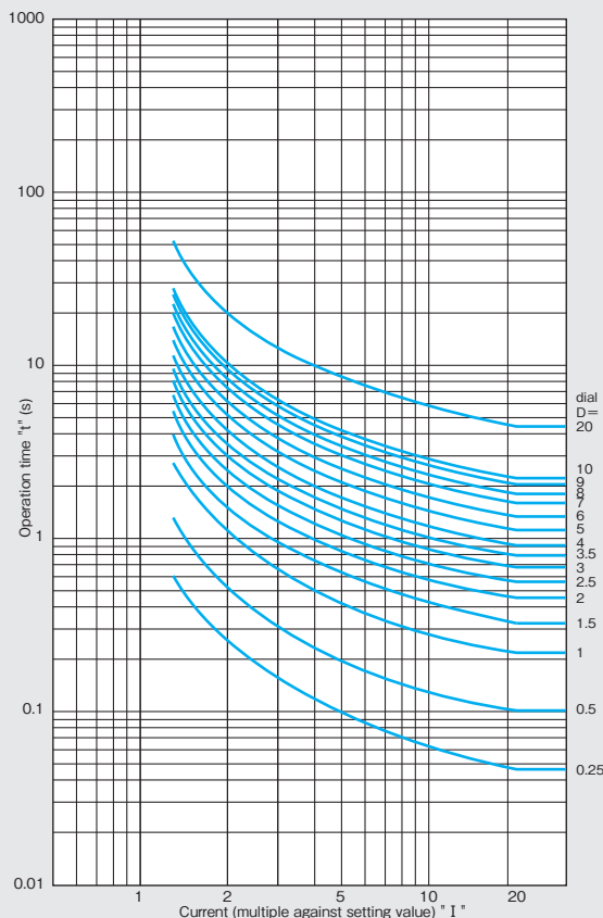
NI : Normal inverse time-delayed characteristic
