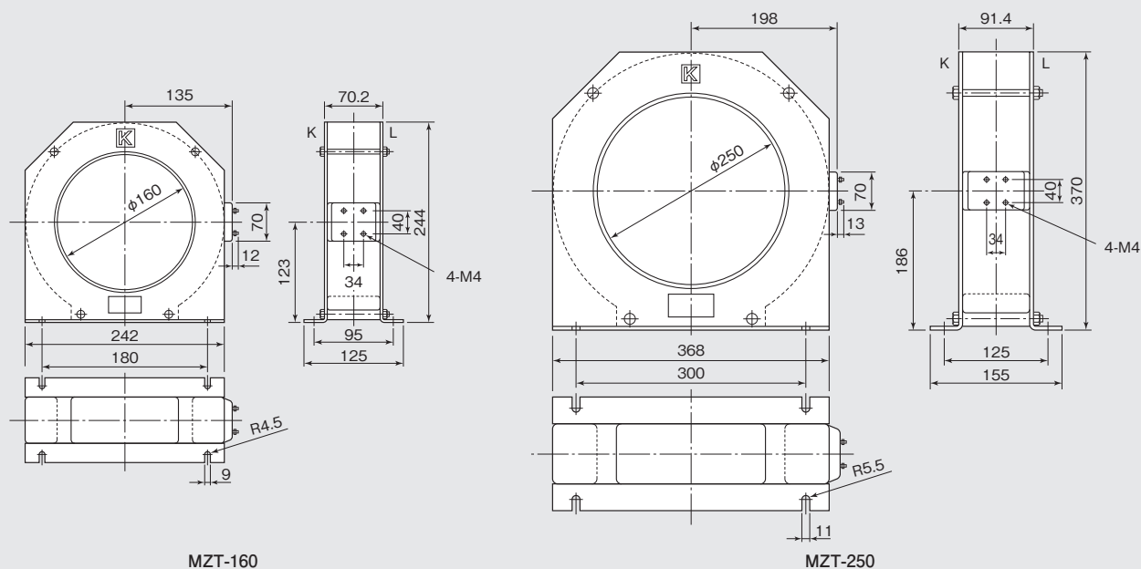
Fig9-5(b) MZT type ZCT (Through type)
