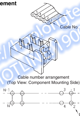
Standard Terminal Arrangement
