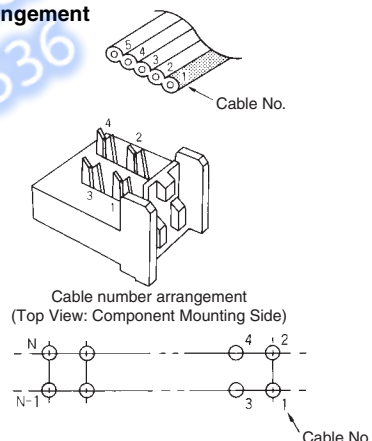
Reverse Terminal Arrangement
