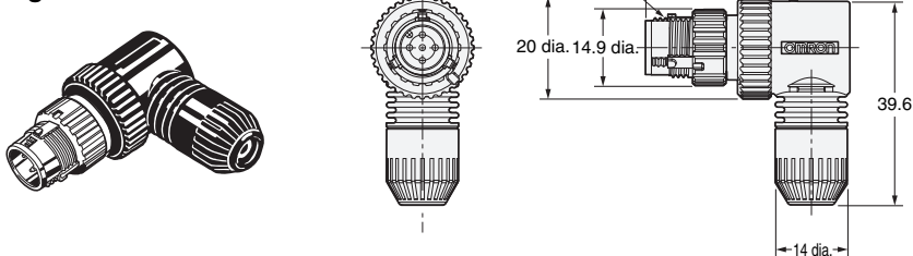
XS5G-D□S□ (Screw-on Connectors) Angled Connectors
