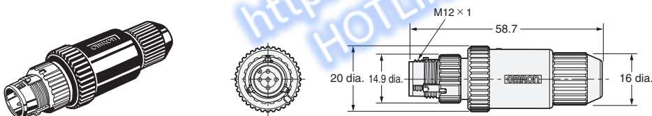
XS5G-D□S□ (Screw-on Connectors, Applicable Cable Outer Diameter: 7 or 8 mm) Straight Connectors
