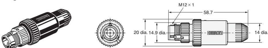
XS5G-D□S□ (Screw-on Connectors, Applicable Cable Outer Diameter: 3, 4, or 6 mm) Straight Connectors
