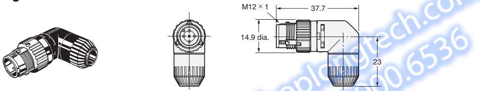
XS5G-D42□ (Soldering Model) Angled Connectors
